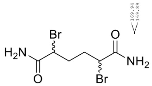
2,5-Dibromohexanediamide (2)
