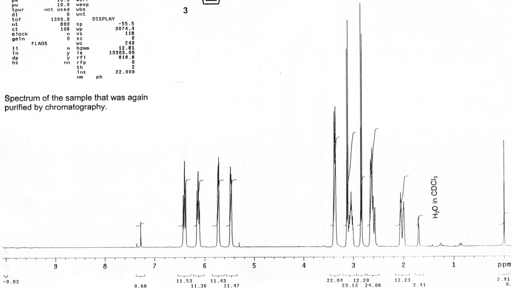
1 H NMR (300MHz, CDCl 3 ) spectrum of 9-Spiroepoxy-endo-tricyclo[5.2.2.0 2,6 ]undeca-4,10-diene-8-one (3)
