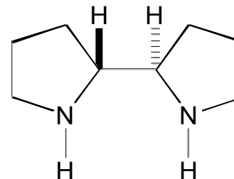
(R,R')-BIS-PYRROLIDINE L-TARTRATE
