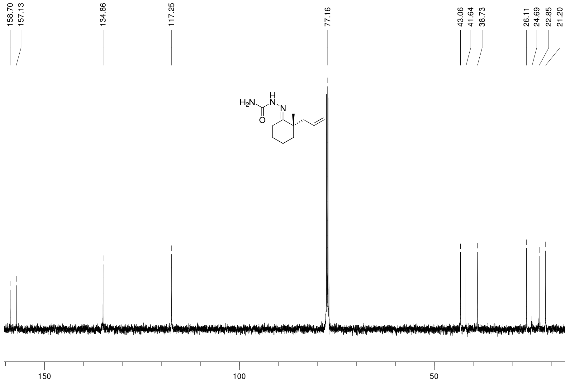
^{13}\text{C} NMR Spectrum of (2E) -2-[( 2S )-2-Methyl-2-(2-propen-1-yl)-cyclohexylidene]hydrazinecarboxamide (101 MHz, \text{CDCl}_3 )
