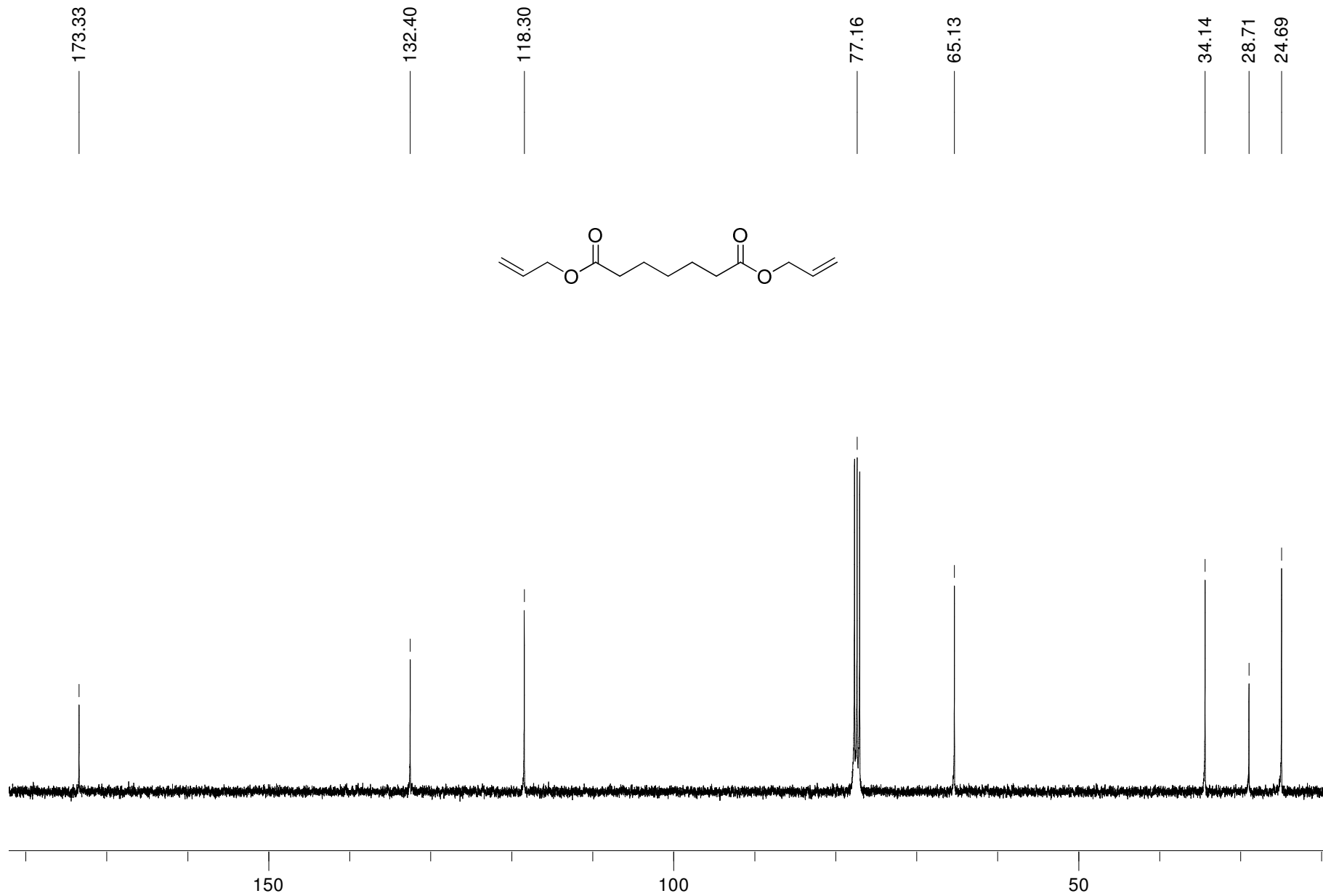
13 C NMR Spectrum of diallyl pimelate (101 MHz, CDCl 3 )
