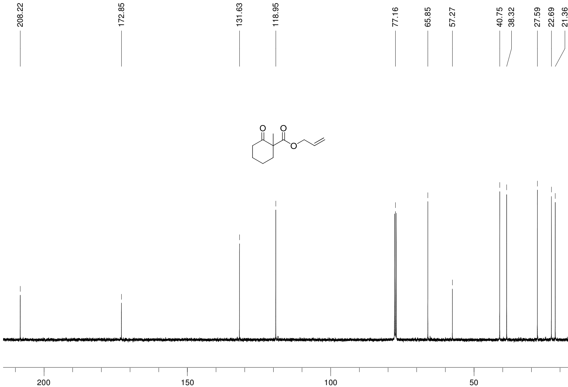
13 C NMR Spectrum of 1Methyl-2-oxo-Cyclohexanecarboxylic acid 2-propenyl ester (101 MHz, CDCl 3 )
