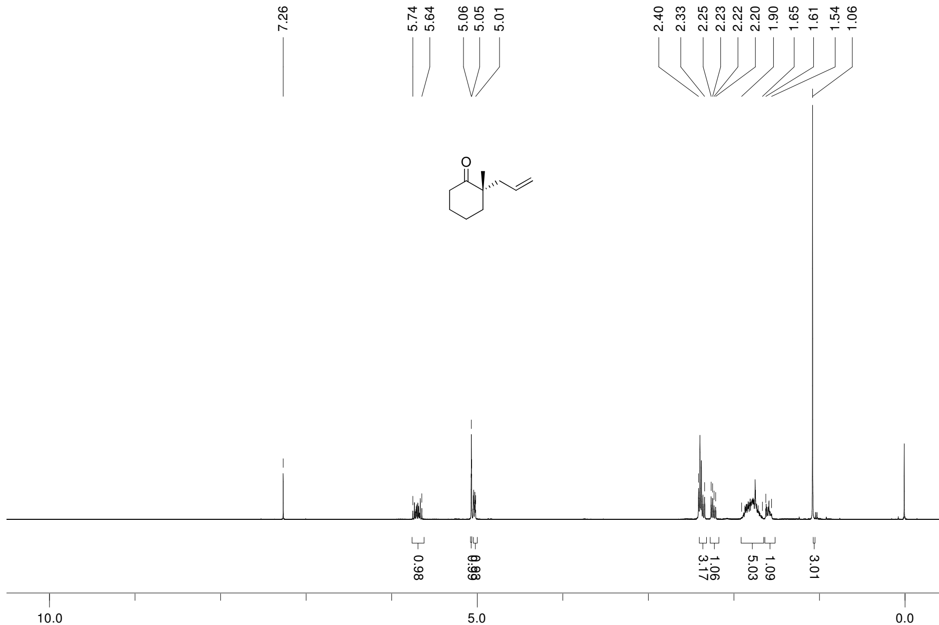
^1\text{H} NMR Spectrum of (2 S )-2-Methyl-2-(2-propen-1-yl)-cyclohexanone (400 MHz, \text{CDCl}_3 )
