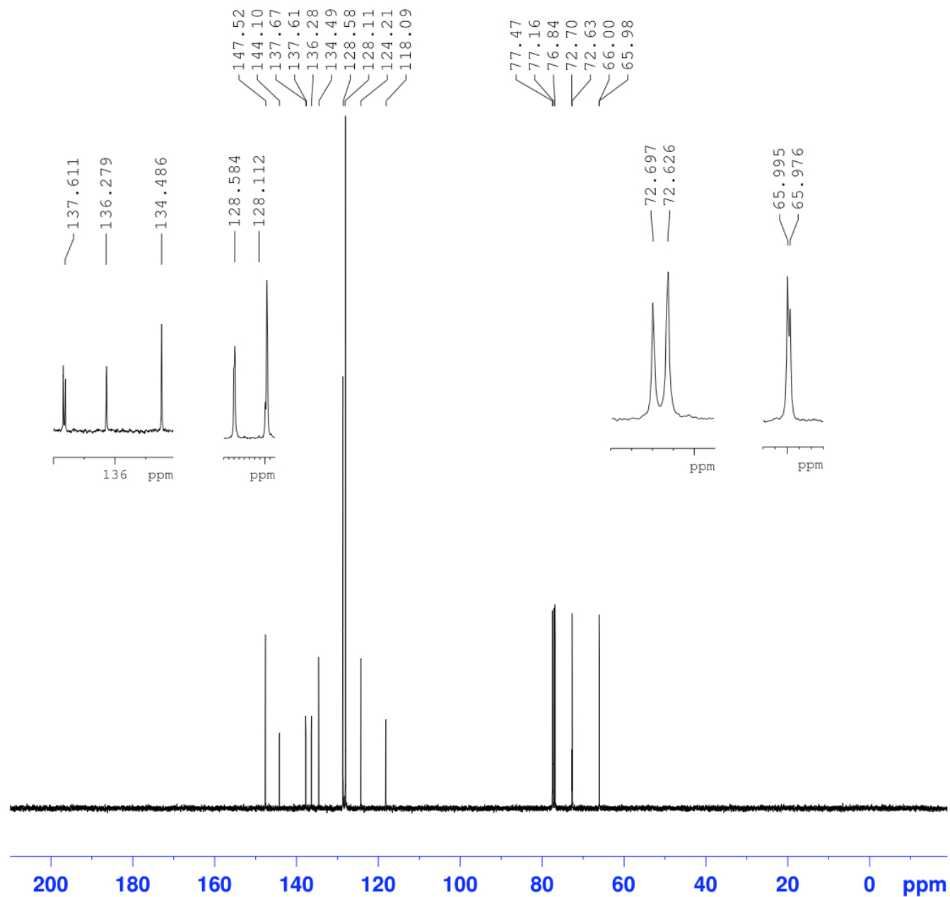
(2Z)-4-(benzyloxy)but-2-enal oxime
