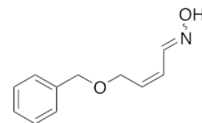
(2Z)-4-(benzyloxy)but-2-enal oxime
