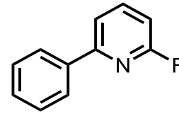
2-fluoro-6-phenylpyridine
