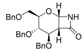
tri-O-Bn-D-glucal- \beta -lactam ( 1 ) ^{13}\text{C} NMR (100MHz, \text{CDCl}_3 )
